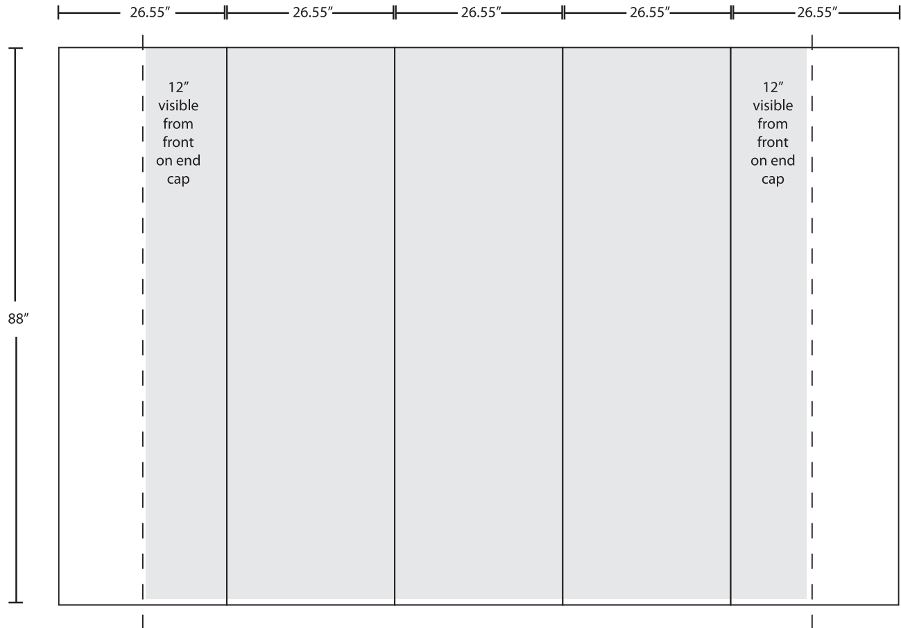
Over head floor plan with curves in place on ends
